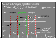
TUB-test chart eeg4; Colour thresholds and colour spaces; antagonistic receptor functions F_{ab} F_{ab} and derivation F'_{ab} , functions e^x with relative luminance x = \log(L/L_a) and contrast range
