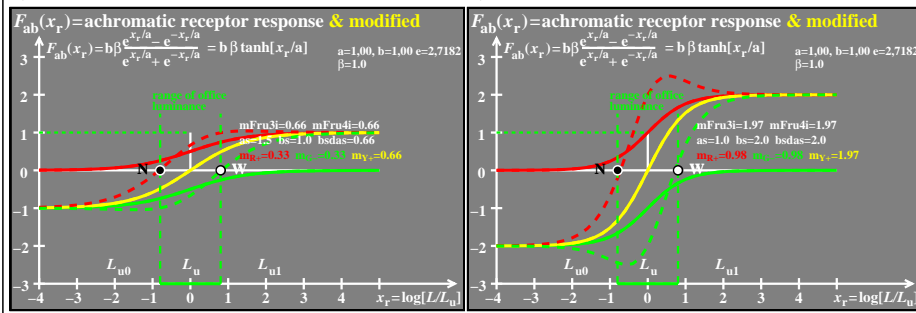
TUB-test chart eej4; TUBJND model of response functions F_{ab}(x_r) , and derivation F'_{ab}(x_r) Receptor response Y+ , and amplitude modulations Y+ \& R+ / G- (left), Y+ \& R+ / G- (right)
