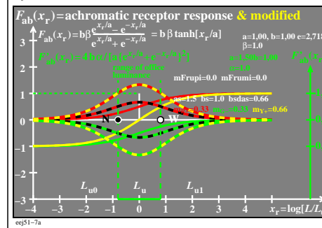
TUB-test chart eej5; TUBJND model of response functions F_{ab}(x_r) , and derivation F'_{ab}(x_r) Receptor responses R_+ , G_- , Y_+ , and derivations Y_+ , Y_- (left & right), and R_+ , G_- (right)
