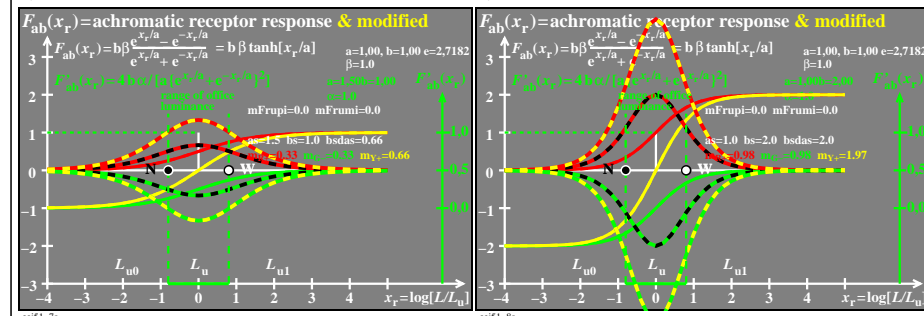
TUB-test chart eej5; TUBJND model of response functions F_{ab}(x_r) , and derivation F'_{ab}(x_r) Receptor responses R_+ , G_- , Y_+ , and derivations Y_+ , Y_- (left & right), and R_+ , G_- (right)
