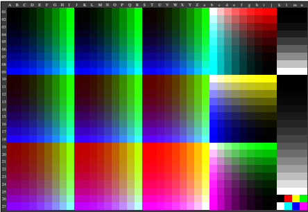
eem41-8A, gamma g_a=5,052 , g_p=2,105 , C_{Yp15}=C_{Yn1}
