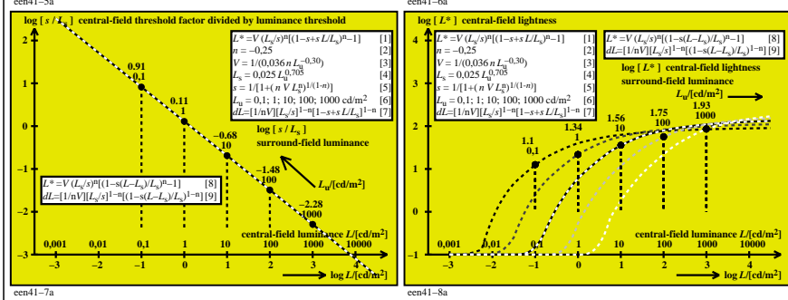
TUB-test chart een4; Achromatic thresholds; 5 luminances L_0=0.1, 1, 10, 100, 1000 \text{ cd/m}^2 \Delta L (0,4s), contrast, and lightness; experimental data of Lingelbach and Richter
