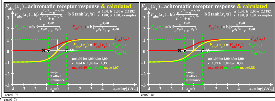
TUB-test chart een6; TUBJND model, lightness F_{abc} , F_{abc,r} , receptor responses F_{ab}(R^+) , F_{cb}(G^-) , F_{ab}+F_{cb}(Y^+) (left), relative responses (right) for parameter a=1 and different b
