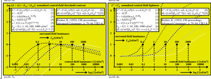
TUB-test chart ees1; Achromatic thresholds; 5 luminances L_0=0.1, 1, 10, 100, 1000 \text{ cd/m}^2 \Delta L (0,4s), contrast, and lightness; experimental data of Lingelbach and equations of Richter
