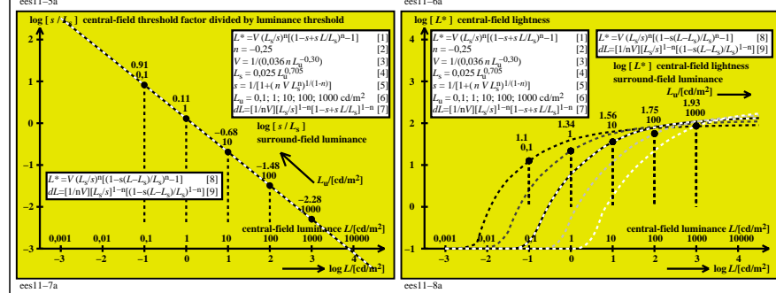
TUB-test chart ees1; Achromatic thresholds; 5 luminances L_u=0,1, 1, 10, 100, 1000 \text{ cd/m}^2 \Delta L (0,4s), contrast, and lightness; experimental data of Lingelbach and equations of Richter
