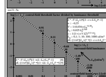
TUB-test chart ees3; Achromatic thresholds; 5 luminances L_0=0.1, 1, 10, 100, 1000 \text{ cd/m}^2 \Delta L (0.4s), contrast, and lightness; experimental data of Lingelbach and equations of Richter
