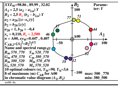
TUB-test chart eet0; Ostwald optimal colours, Yw=90 & 100, D65, D50, P40, A00, CIE-02-degree Antagonistic hue circle, approximately constant chromatic value CAB,2 for contrast C=>288:1
