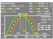
TUB-test chart eeV1; Cone sensitivities of the antagonistic TUBLAB colour-vision model linear and log sensitivity and saturation of TUBLAB-model cones L & M
