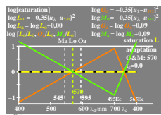
TUB-test chart eeV1; Cone sensitivities of the antagonistic TUBLAB colour-vision model linear and log sensitivity and saturation of TUBLAB-model cones L & M
