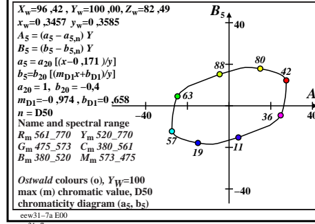
TUB-test chart eew3; CIE (x, y) and chromatic values (A i , B i ), Oswald optimal colours for the illuminants D65 and D50; chromatic-value diagrams for these illuminants, Y w =100
