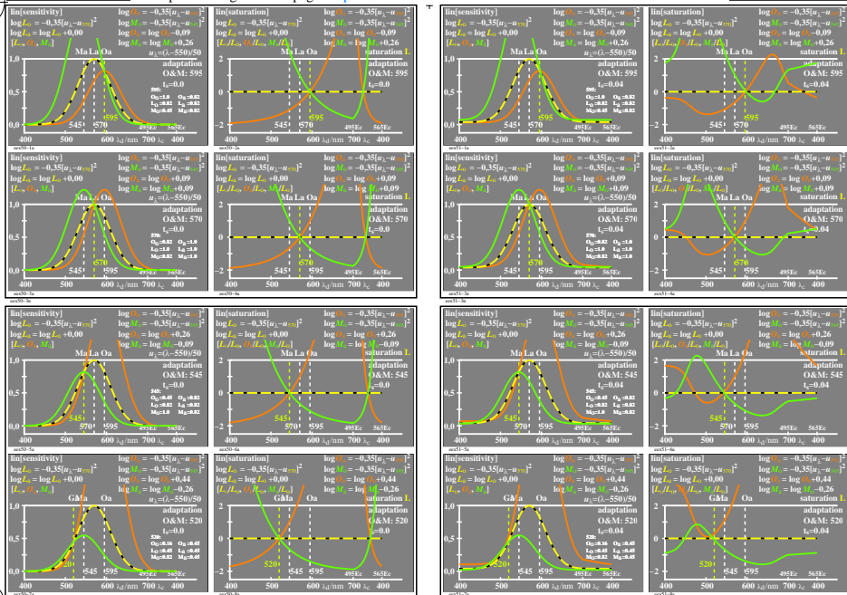
TUB-test chart eex5; sensitivity LMO→M/L & O/L, lin[thresholds]=0 & 0.04 lin[sensitivity] and lin[ratio], LMS-R21, 4 adaptations: 595,570,545,520
