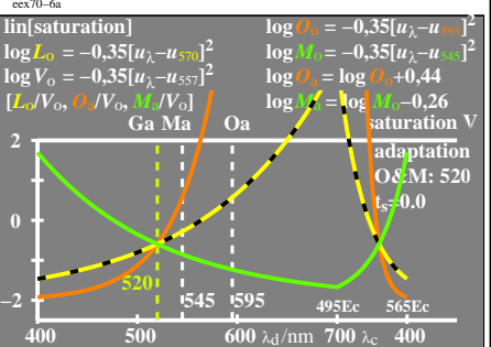
TUB-test chart eex7; sensitivity LMO→L/V & O/V, lin[thresholds]=0 & 0,04 lin[sensitivity] and lin[ratio], LMS-R21, 4 adaptations: 595,570,545,520
