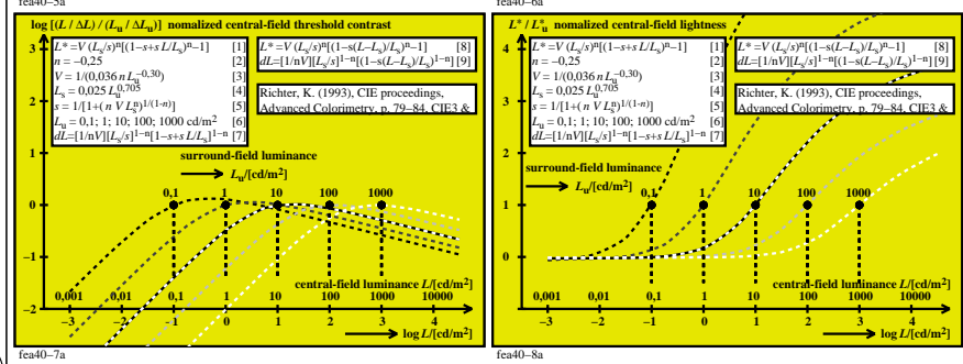
TUB-test chart fea4; Achromatic thresholds; 5 luminances L_U=0,1, 1, 10, 100, 1000 \text{ cd/m}^2 \Delta L (0,4s), contrast, and lightness; experimental data of Lingelbach and equations of Richter
