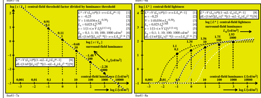
TUB-test chart fea4; Achromatic thresholds; 5 luminances L_U=0,1, 1, 10, 100, 1000 \text{ cd/m}^2 \Delta L (0,4s), contrast, and lightness; experimental data of Lingelbach and equations of Richter
