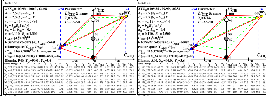
TUB-test chart fec6; Ostwald optimal colours, Yw=100, D65, D50, P40, A00, CIE-02-degree, YB constant chromatic value CAB2, contrasts C=>288:1(100:0), 25:1(90:3.6), 16:1(72:4.5), 9:1(54:6), L*
