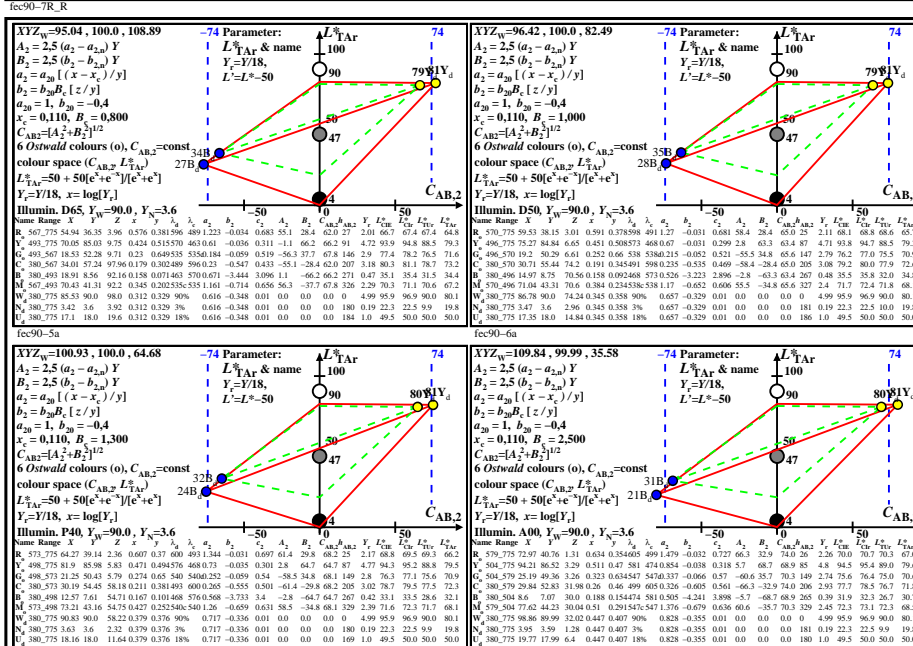
TUB chart fec9; Ostwald optimal colours, Y_w=100, D65, D50, P40, A00, CIE-02\text{-}deg, YB constant chromatic value C_{AB,2} > 288:1(100:0), 25:1(90:3.6), 16:1(72:4.5), 9:1(54:6), L^*
