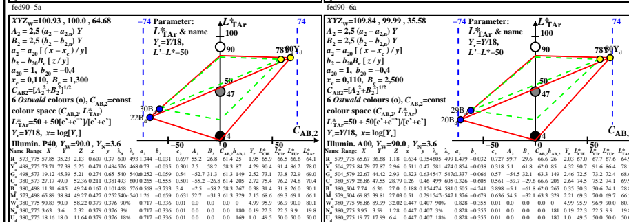
TUB-test chart fed9: Ostwald optimal colours, Y_W = 100.0, D65, D50, P40, A00, CIE-02 -degree, YB constant chromatic value CAB,2 , contrasts C > 288:1 (100:0), 25:1 (90:3.6), 16:1 (72:4.5), 9:1 (54:6), L^*
