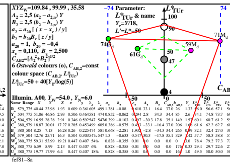
TUB-test chart feF8; 6 Ostwald optimal colours, Y_w=100, D65, D50, P40, A00, CIE-02 -degree, YB constant chromatic value CAB_2 , contrasts C=>288:1(100:0), 25:1(90:3:6), 16:1(72:4:5), 9:1(54:6), L^*
