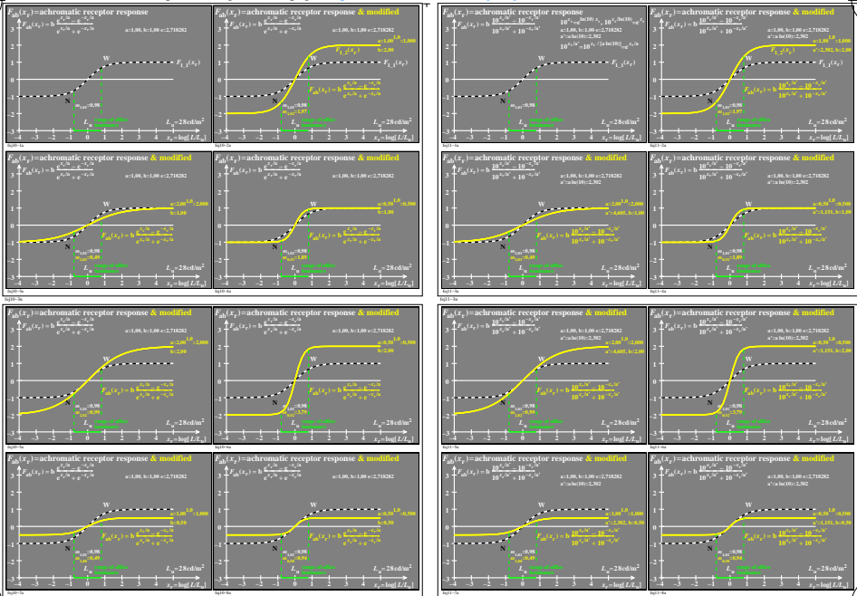
TUB-test chart fej1; Model of achromatic response functions F_{ab}(x_r) , visual processes N, W, N+W Tangens hyperbolicus \tanh(x_r) and modified with e^{x_r/a} and 10^{x_r/a} ; a = a \ln(10)
