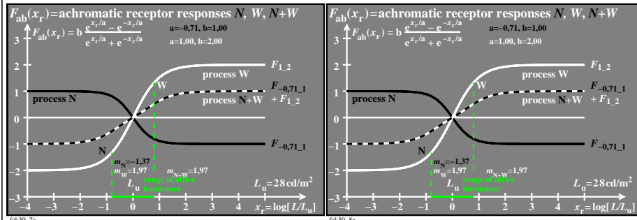
TUB-test chart fek3; Model of response functions F_{ab}(x_r) , processes N, W, N+W Tangens hyperbolicus \tanh(x_r) and modified with e^{\pm x_r/a} and 10^{\pm x_r/a} ; a=-0,71 & 1,00 ; a' = a \ln(10)
