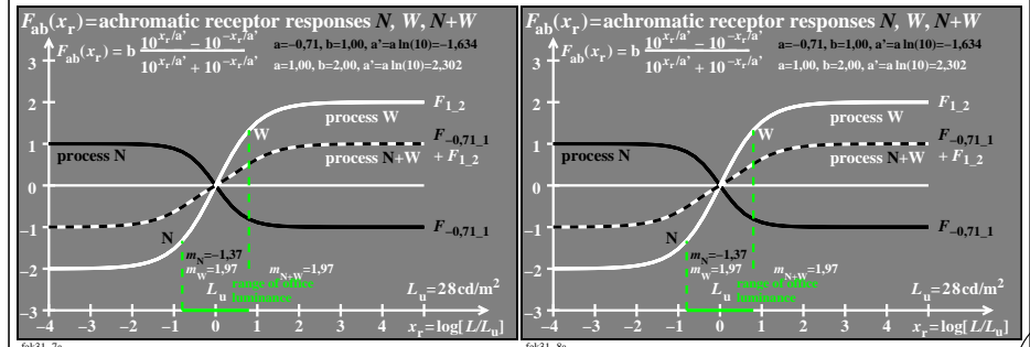
TUB-test chart fek3; Model of response functions F_{ab}(x_r) , processes N, W, N+W Tangens hyperbolicus \tanh(x_r) and modified with e^{\pm x_r/a} and 10^{\pm x_r/a} ; a=-0,71 & 1,00 ; a' = a \ln(10)
