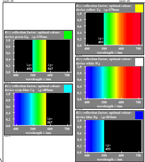
Wavelength ranges for CIE standard illuminant D65
