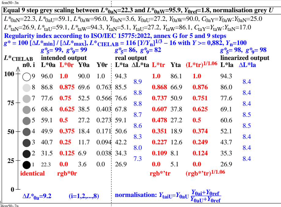
TUB-test chart fem5; Equal 9 step grey scaling for four display reflections Y_{ref}=3.6, 1.8, 0.9, 90 , and black L^*_{N,CIELAB}=22.3 , Y_N=3.6 and white L^*_{W,CIELAB}=95.99 , Y_W=90 , normalisation: grey U
