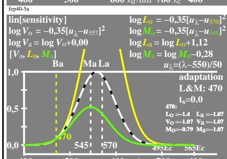
TUB-test chart fep4; sensitivity LMS-R24, 4 adaptations: 620,570,520,470 lin[sensitivity] and lin[ratio], LMS-R24, 4 adaptations: 620,570,520,470
