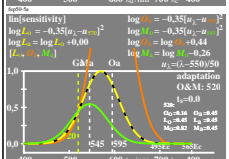
TUB-test chart fep5: sensitivity LMO->M/L & O/L, lin[thresholds]=0 & 0,04 lin[sensitivity] and lin[ratio], LMS-R24, 4 adaptations: 595,570,545,520
