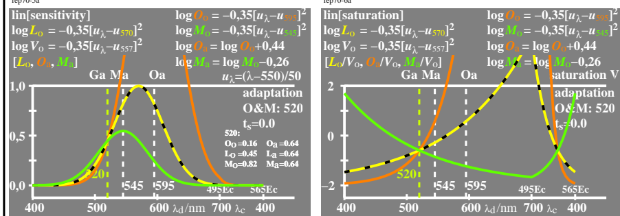
TUB-test chart fep7; sensitivity LMO→L/V & O/V, lin[thresholds]=0 & 0,04 lin[sensitivity] and lin[ratio], LMS-R24, 4 adaptations: 595,570,545,520
