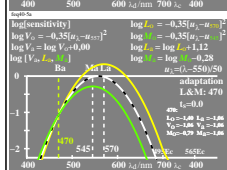
TUB-test chart feq4: sensitivity LMV->L/V & M/V, lin[thresholds]=0 & 0.04 log[sensitivity] and log[ratio], LMS-R24, 4 adaptations: 620,570,520,470
