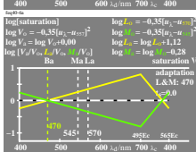
TUB-test chart feq4: sensitivity LMV->L/V & M/V, lin[thresholds]=0 & 0.04 log[sensitivity] and log[ratio], LMS-R24, 4 adaptations: 620,570,520,470
