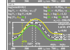
TUB-test chart feq4: sensitivity LMV->L/V & M/V, lin[thresholds]=0 & 0.04 log[sensitivity] and log[ratio], LMS-R24, 4 adaptations: 620,570,520,470
