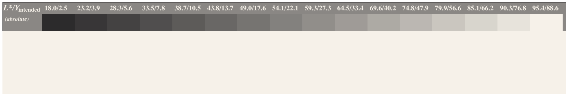
Picture C3: 16 visual equidistant L^* -grey steps; PS operator: 000n* setcmykcolor; use file www.bam.de/FE86/10L/L86E0iFA.PS or L86E0iFP.PS/.PDF (i=0,7) for PDF systems to complete the figure
