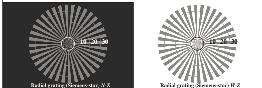
Picture C1: Radial gratings (Siemens-stars) N-W, W-N, N-Z and W-Z; PS operator: 000n* setcmykcolor
