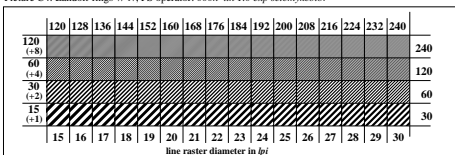
Picture C5: Line raster under 45° (or 135°); PS operator: 000n*lin 1.0 exp setcmkycolor
