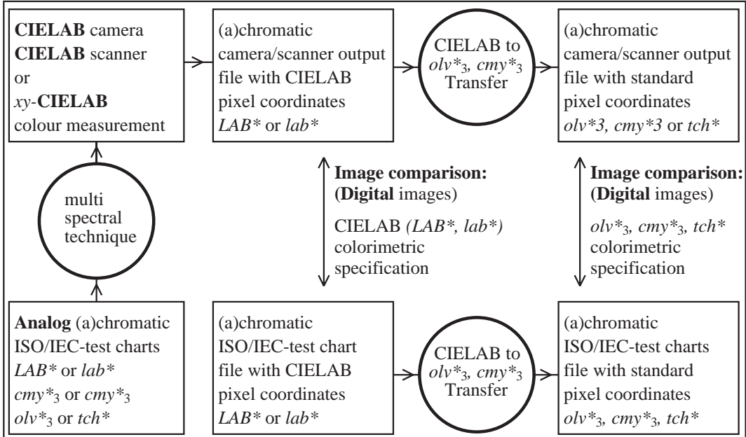
LE430-7, Transfer from device independent data LAB^* to device dependent data olv^*_3, cmy^*_3 and tch^*
