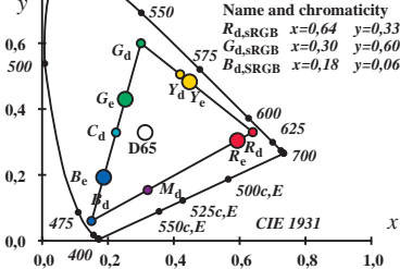
Device and elementary colours of the sRGB colour space for D65, Y_W=88,6 in the chromaticity diagram ( x, y )
