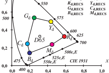
CIE data for device colours (offset of maximum (m) C_{AB} for D65 in the chromaticity diagram ( x, y ))
