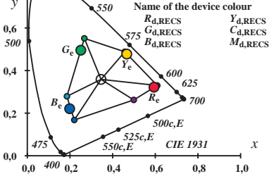
Device and elementary colours of the offset colour space for D50, Y_W=100 in the chromaticity diagram ( x, y )
