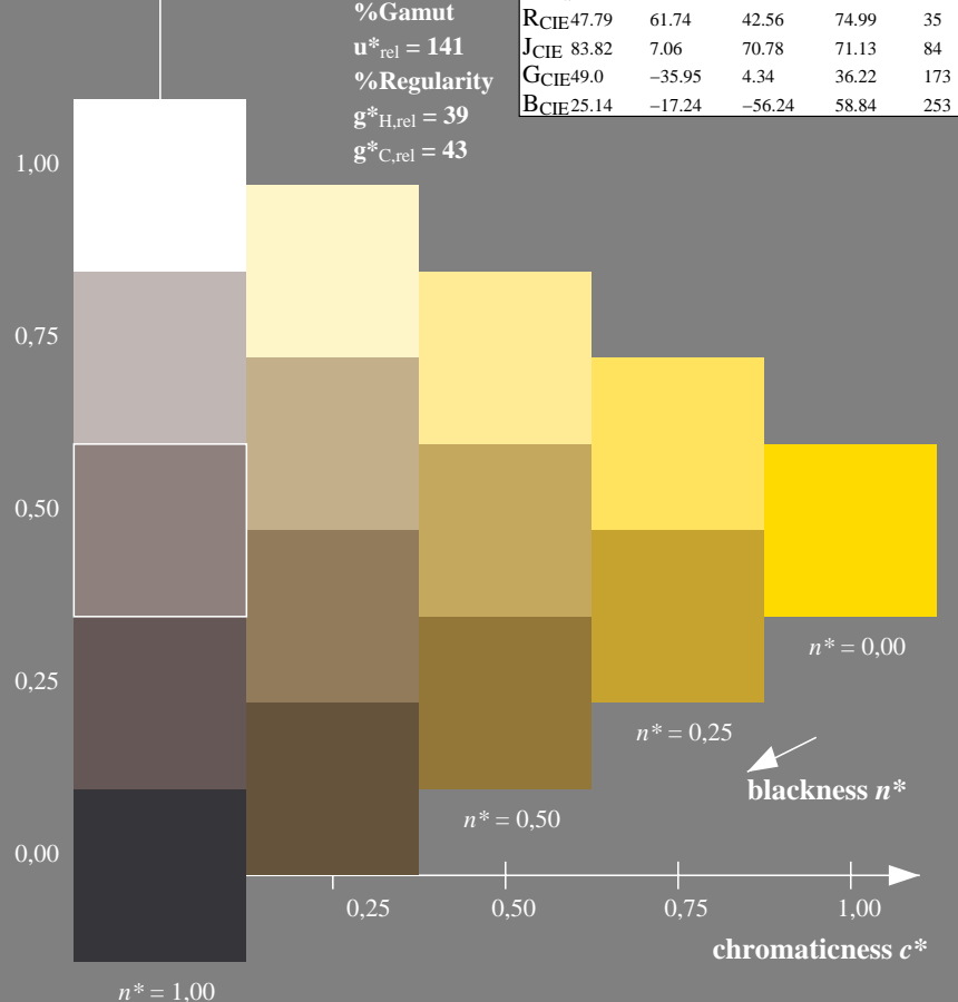
5 step scales for constant CIELAB hue 84/360 = 0.234 (right)
