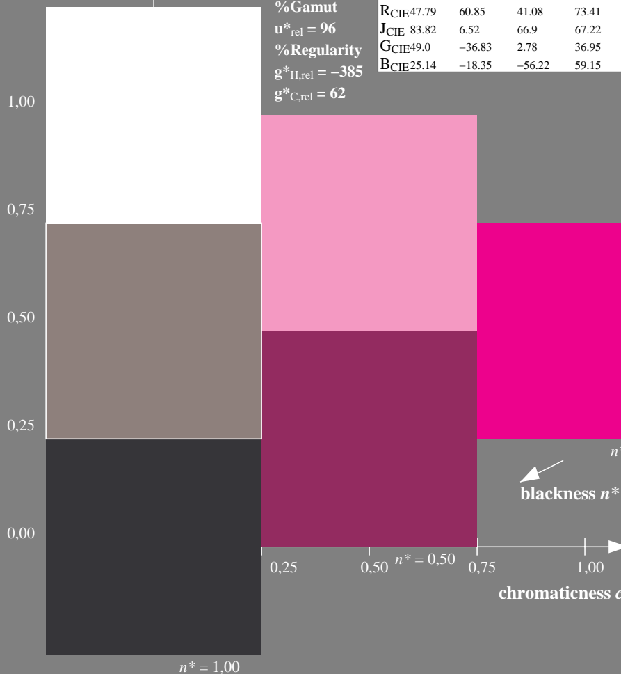
SE800-7, 3 step scales for constant CIELAB hue 6/360 = 0.017 (left)
