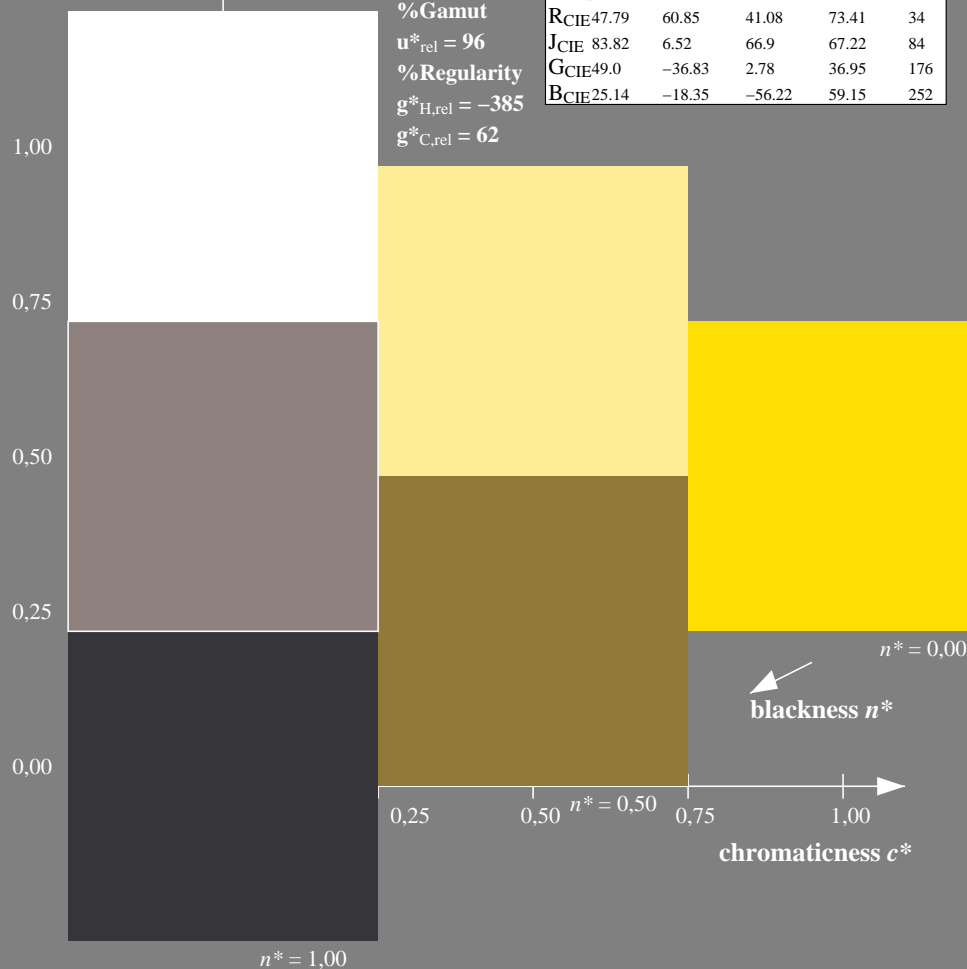
SE800-7, 3 step scales for constant CIELAB hue 84/360 = 0.235 (left)
