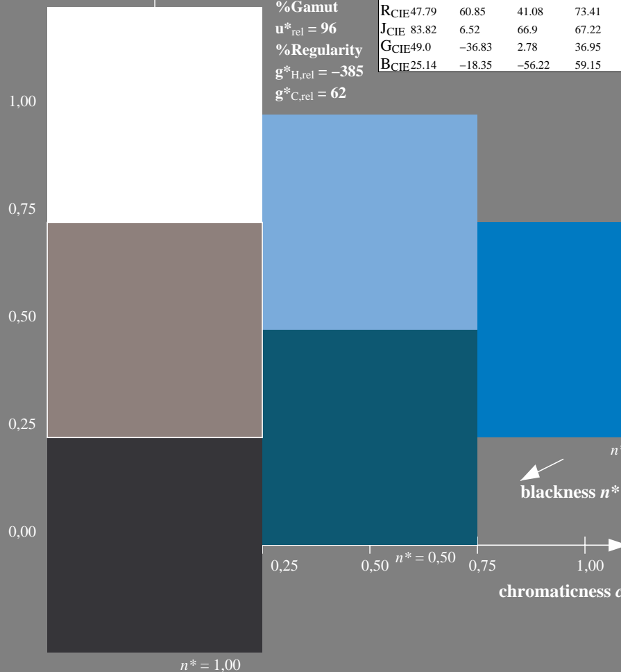
SE800-7, 3 step scales for constant CIELAB hue 252/360 = 0.7 (left)
