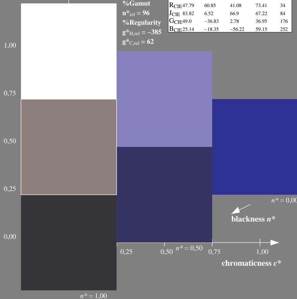
SE800-7, 3 step scales for constant CIELAB hue 304/360 = 0.845 (left)
