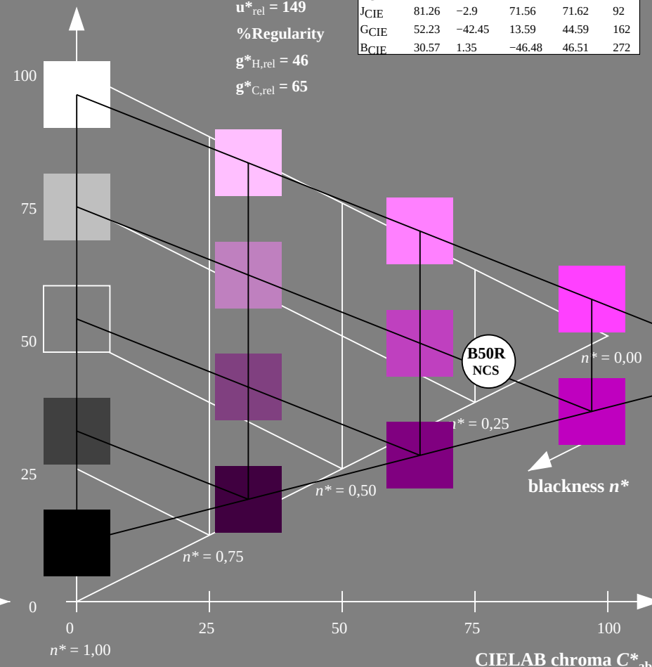
5 step scales for constant CIELAB hue 325/360 = 0.903 (right)
