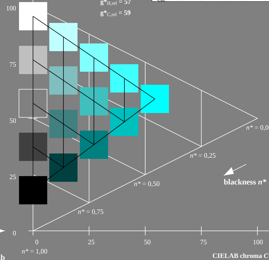
5 step scales for constant CIELAB hue 236/360 = 0.656 (right)
