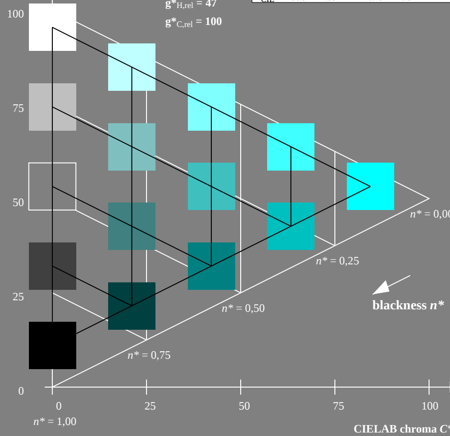
TE370-7, 5 step scales for constant CIELAB hue 203/360 = 0.564 (left)
