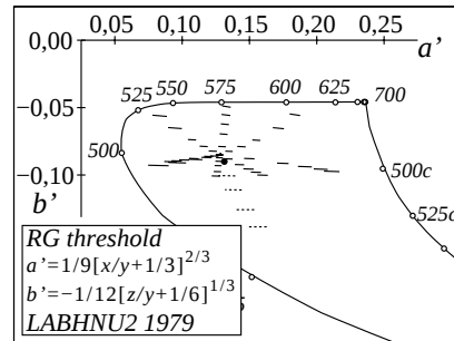
WE550-6, Colours in (a',b') colour diagram
