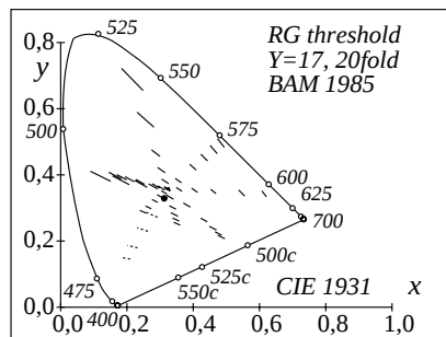
WE550-1, Colours in (x,y) chromaticity diagram
