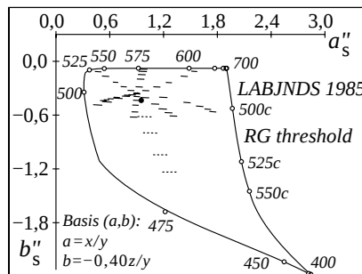
WE550-7, Colours in (a'',b'') colour diagram
