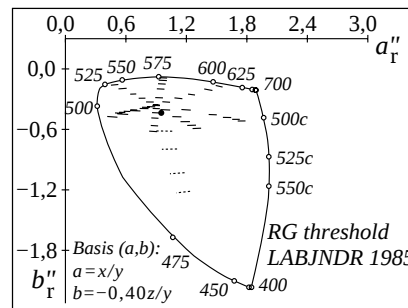
WE550-8, Colours in (a'',b'') colour diagram
