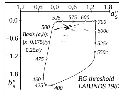
WE551-7, Colours in (a'',b'') colour diagram
