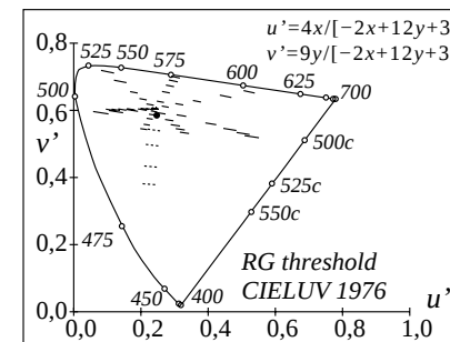
WE551-2, Colours in (u',v') chromaticity diagram
