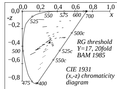
WE551-1, Colours in (x,-z) chromaticity diagram
