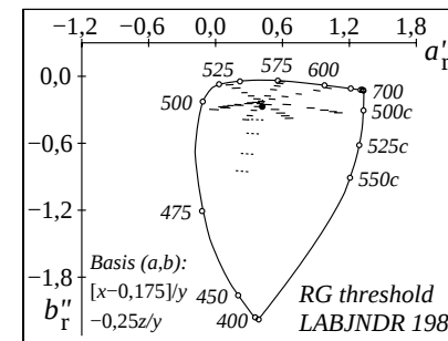
WE551-8, Colours in (a'',b'') colour diagram
