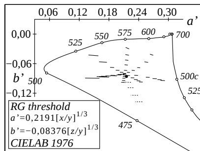
WE550-3, Colours in (a',b') colour diagram
