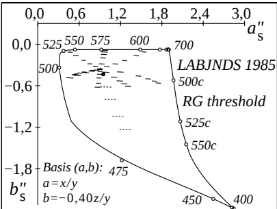
WE550-7, Colours in ( a''_s, b''_s ) colour diagram
