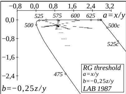
WE551-3, Colours in (a,b) chromaticity diagram
