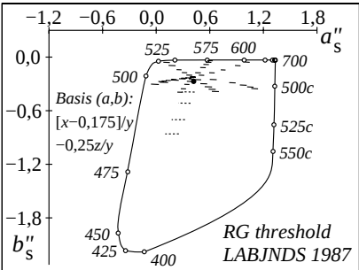
WE551-7, Colours in ( a''_s, b''_s ) colour diagram
