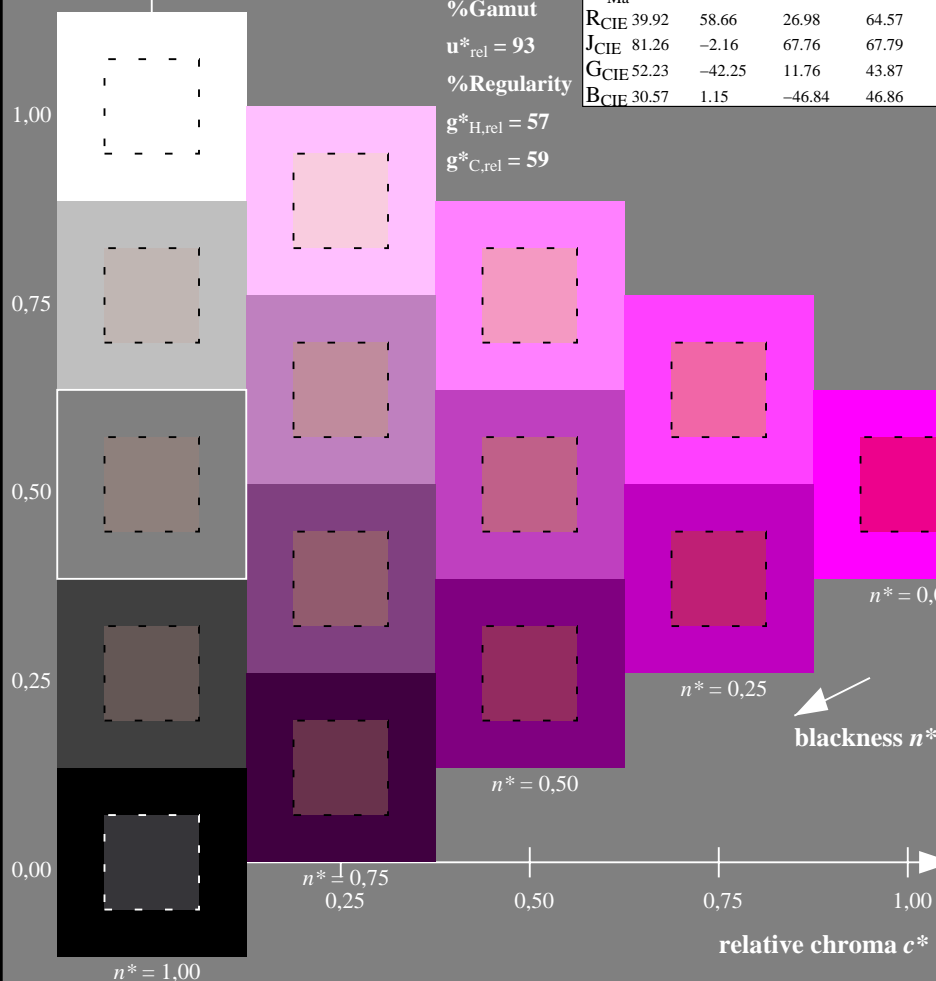
De140-7N, 5 step scales for constant CIELAB hue 354/360 = 0.982 (left)
