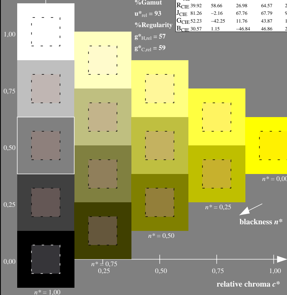
De140-7N, 5 step scales for constant CIELAB hue 96/360 = 0.268 (left)
