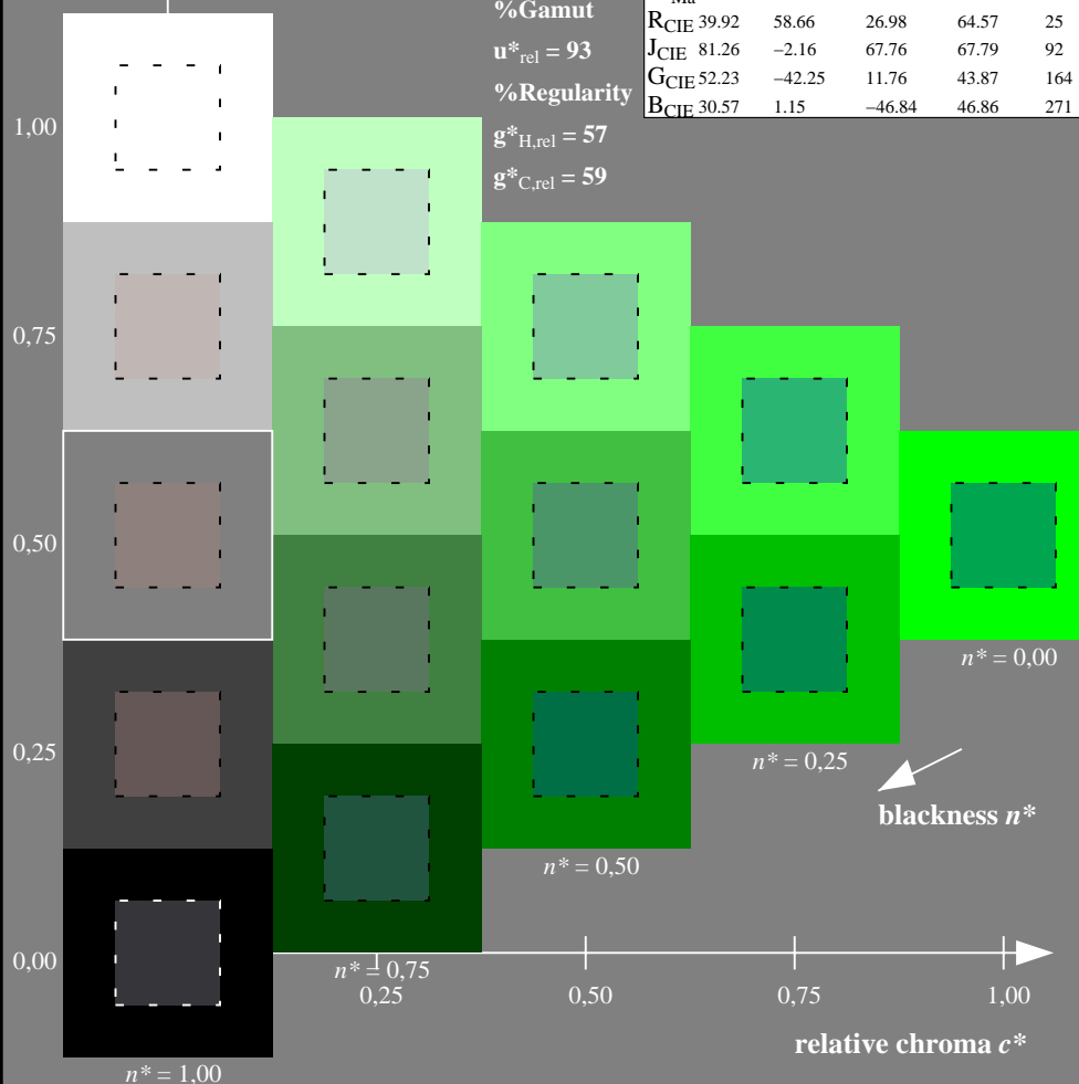
De140-7N, 5 step scales for constant CIELAB hue 151/360 = 0.419 (left)
