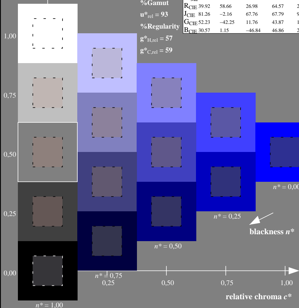
De140-7N, 5 step scales for constant CIELAB hue 305/360 = 0.847 (left)
