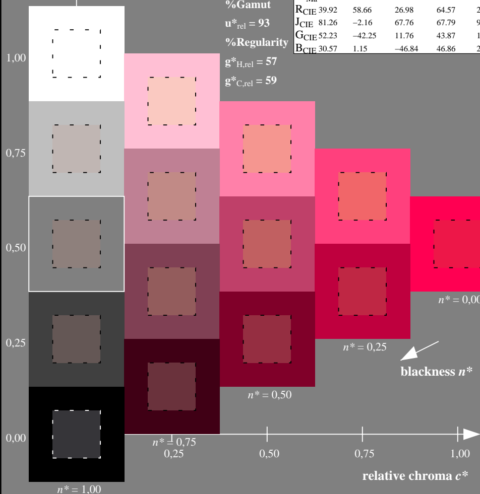
De140-7N, 5 step scales for constant CIELAB hue 25/360 = 0.069 (left)
