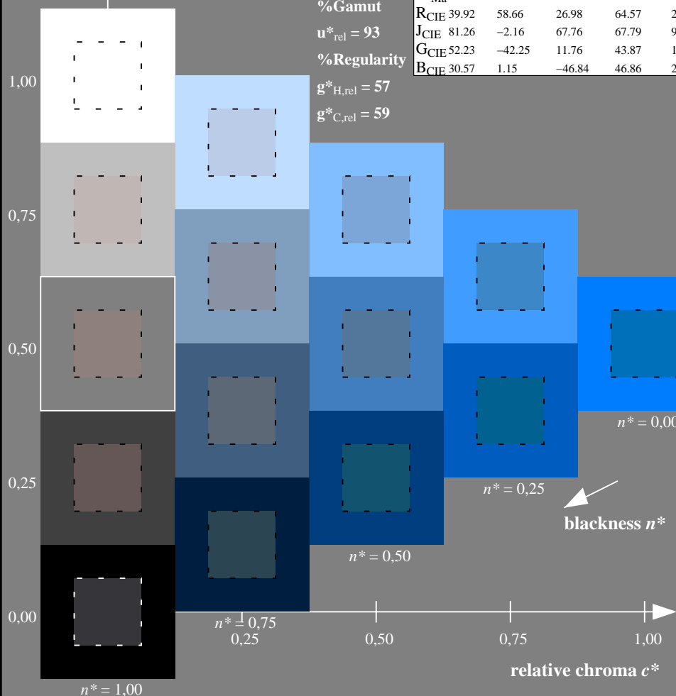
De140-7N, 5 step scales for constant CIELAB hue 271/360 = 0.754 (left)
