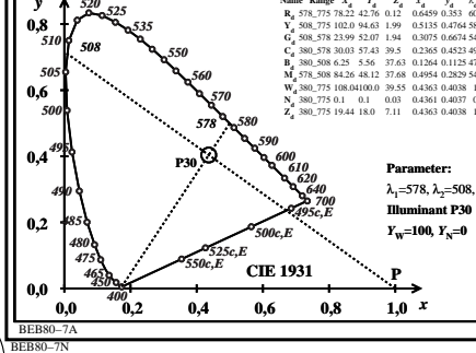
TUB-test chart BEB8; 6 Ostwald optimal colours for 8 illuminants Pxx input: rgb/cmy0/000k/n (left) and Dxx (right), (x, y)_{400,700} , lines separate wavelength ranges of Ostwald optimal colours
