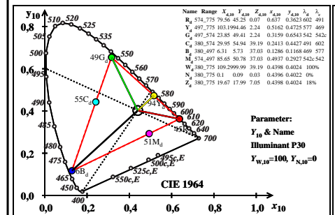
TUB-test chart BED0; 6 Ostwald optimal colors for 8 illuminants Pxx, input: rgb/cmy0/000k/n CIE-10, diagrams (x 10 , y 10 ), C>288:1
