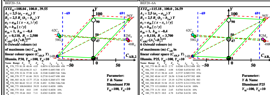
TUB-test chart BEF2; 6 Ostwald optimal colours for 8 illuminants Pxx, input: rgb/cmy0/000k/n CIE-02, diagrams (C_AB,2, Y), C=10=1 to 100, antagonistic reflection
