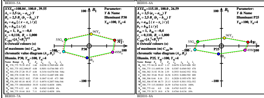
TUB-test chart BEH1; 6 Ostwald optimal colours for 8 illuminants Pxx, input: rgb/cmy0/000k/n CIE-02, diagrams (A1, B1) & (A2, B2), C=25:1
