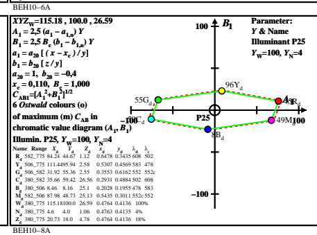
TUB-test chart BEH1; 6 Ostwald optimal colours for 8 illuminants Pxx, input: rgb/cmy0/000k/n CIE-02, diagrams (A1, B1) & (A2, B2), C=25:1
