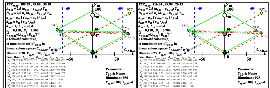
TUB-test chart BEK1; 6 Ostwald optimal colours for 8 illuminants Pxx, input: rgb/cmy0/000k/n CIE-10, diagrams (C_{AB,2,10}, Y_{10}) , C=25:1 , scale Y_{10}=0 to 100 , antagonistic reflection
