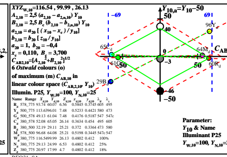
TUB-test chart BEO3; 6 Ostwald optimal colours for 8 illuminants Pxx, input: rgb/cmy0/000k/n CIE-10, diagrams (CAB,2,10, Y10), C=4:1, scale Y10=-50 to 50, antagonistic reflection
