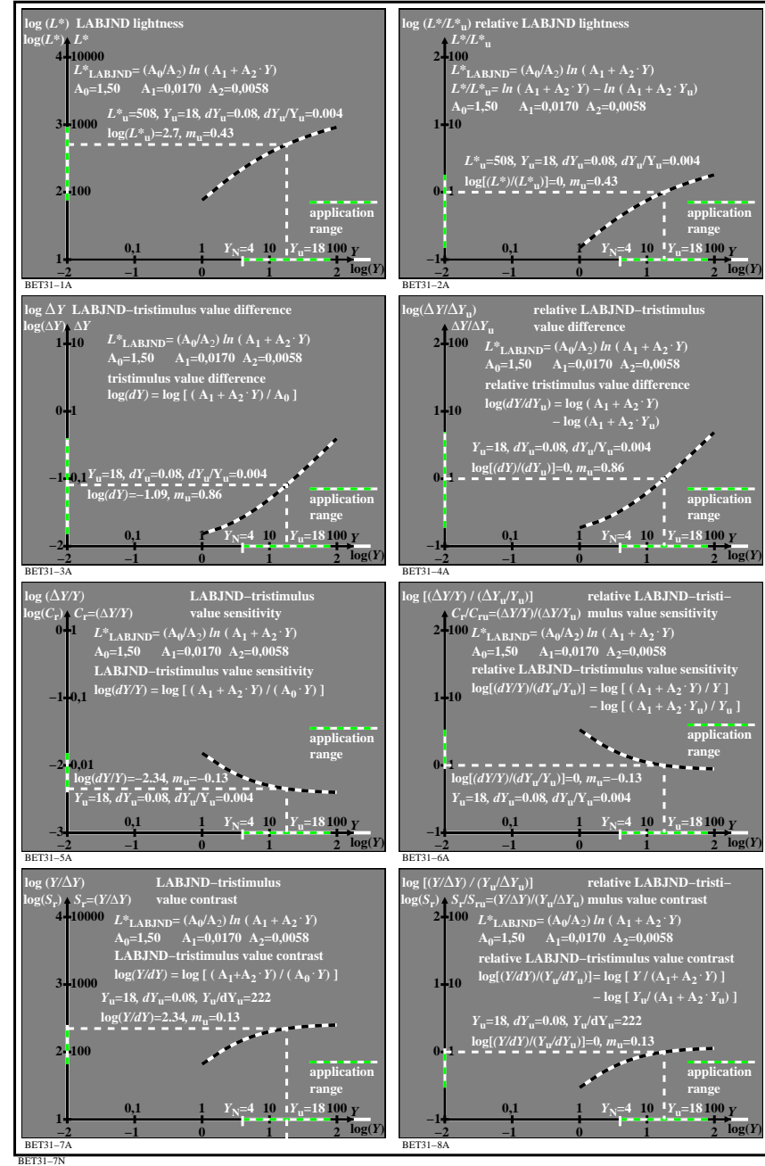
TUB-test chart BET3; CIELAB and LABJND color-difference formulae input: w/rgb Absolute and relative lightness, sensitivity and contrast; colour line element and derivation
