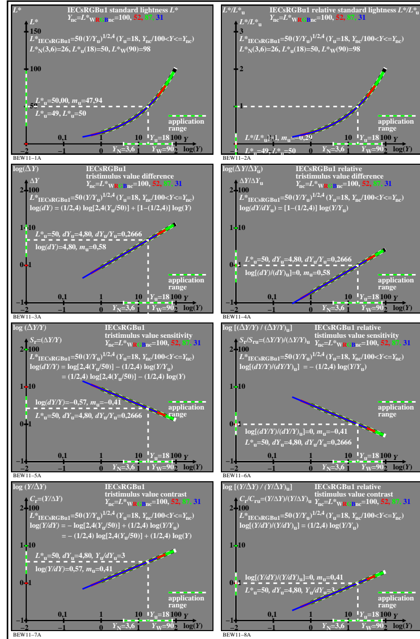
TUB-test chart BEW1; IECsRGBu1, l^* & L^* for Y/Y_u, Y_{nc}=(Y \& L^*)W_{nc} Absolute and relative lightness, sensitivity and contrast, S_n=50,00, 1/\gamma=1/2,4=0,41
